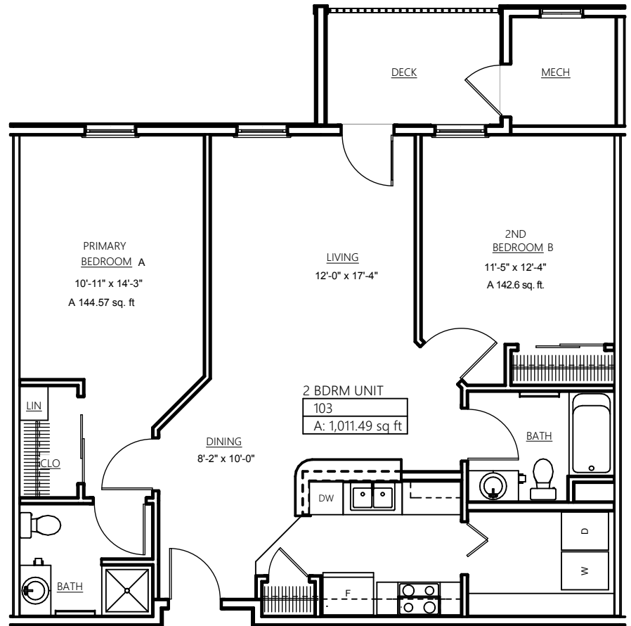
TWO BEDROOM UNIT MIDDLE NTS
